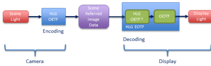
Hybrid Log-Gamma End-to-End Chain
