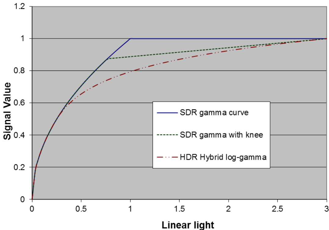
Figure 3: Hybrid log-gamma and SDR OETFs
