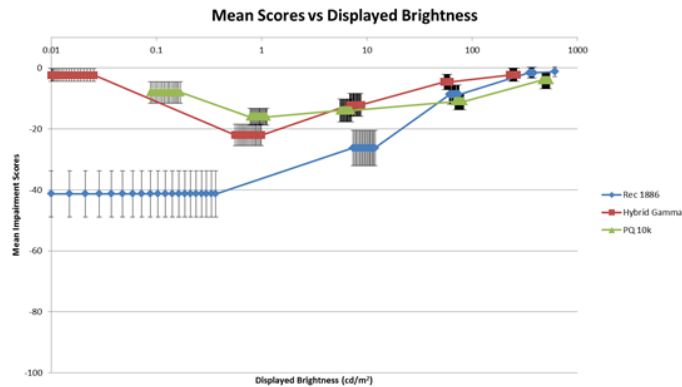
Banding impairment versus displayed brightness
