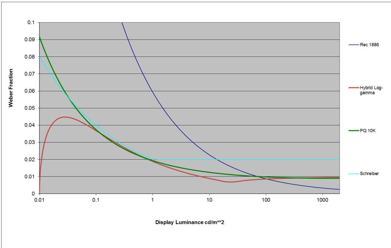
Figure 5: Weber fractions versus display luminance
