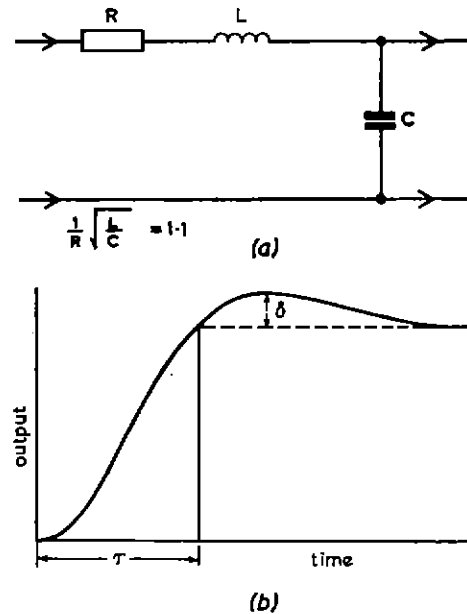
Fig. 10 — Step-shaping network
