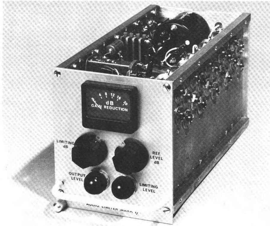
Fig. 12(a) — Experimental limiter; external view
